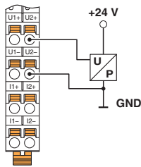
Differential voltage input with active 3-conductor transmitter
